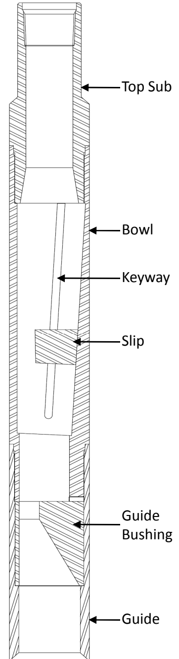
Oversocket Assembly
